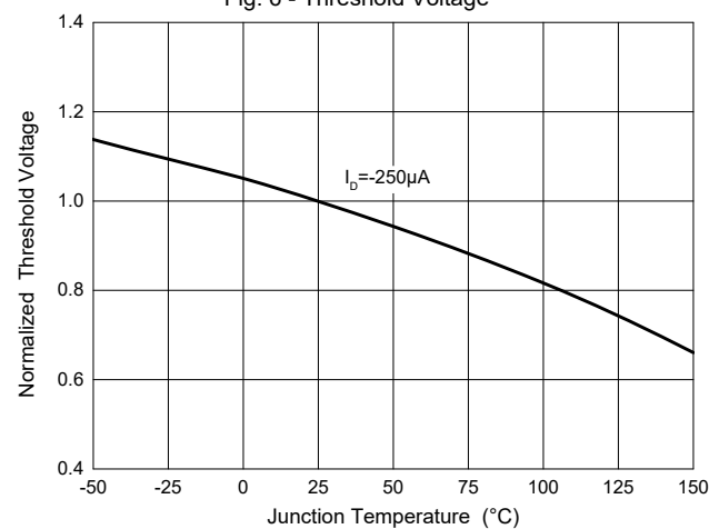
Fig. 6 - Threshold Voltage
